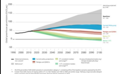
Effect of current pledges and policies on global temperature
